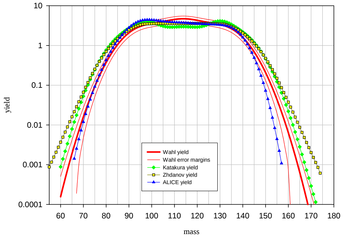
Benchmark B: ^{237}\text{Np} at 100 MeV, post neutron emission yields
